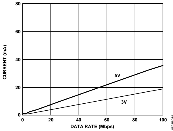
Figure 14. Typical ADuM3401 V_{DD2} Supply Current vs. Data Rate for 5 V and 3 V Operation
